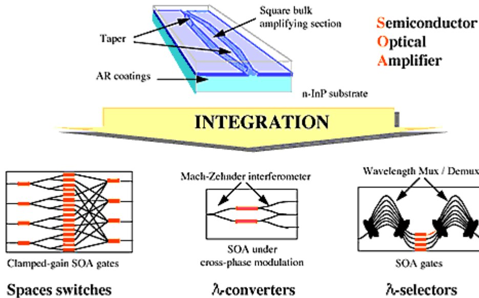
Figure 10: All-Optical Semiconductor Wavelength Converter
