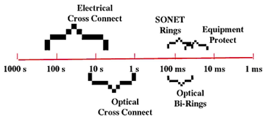
Figure 15: Optical Reconfiguration Performance
